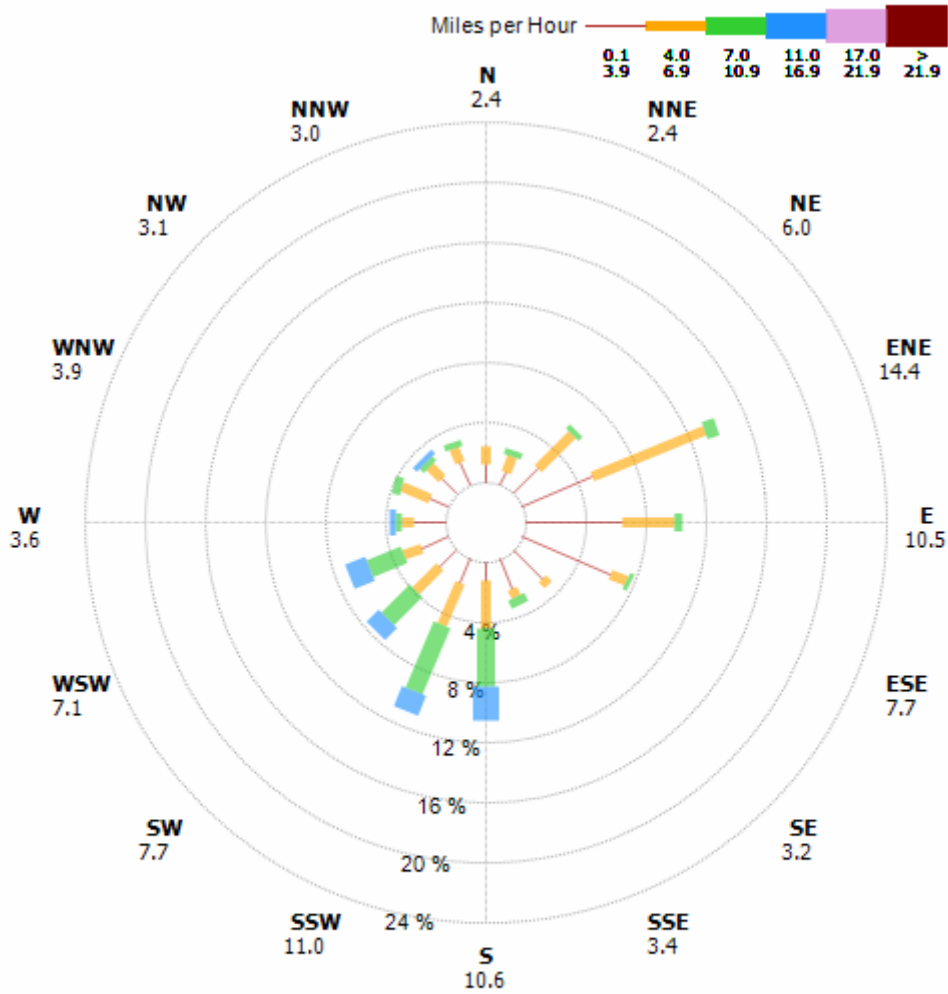
Hour Average Wind Speed Spokane E Ferry ~ 744 Observations 01 Aug 2006 through 31 Aug 2006
