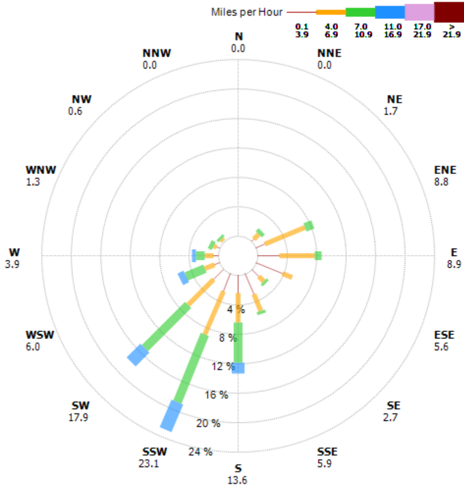
Hour Average Wind Speed Spokane E Ferry ~ 697 Observations 01 Jun 2007 through 30 Jun 2007
