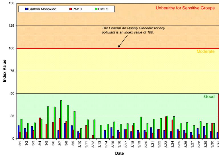
Figure 1: Air Quality Index (AQI) values for March 2011
