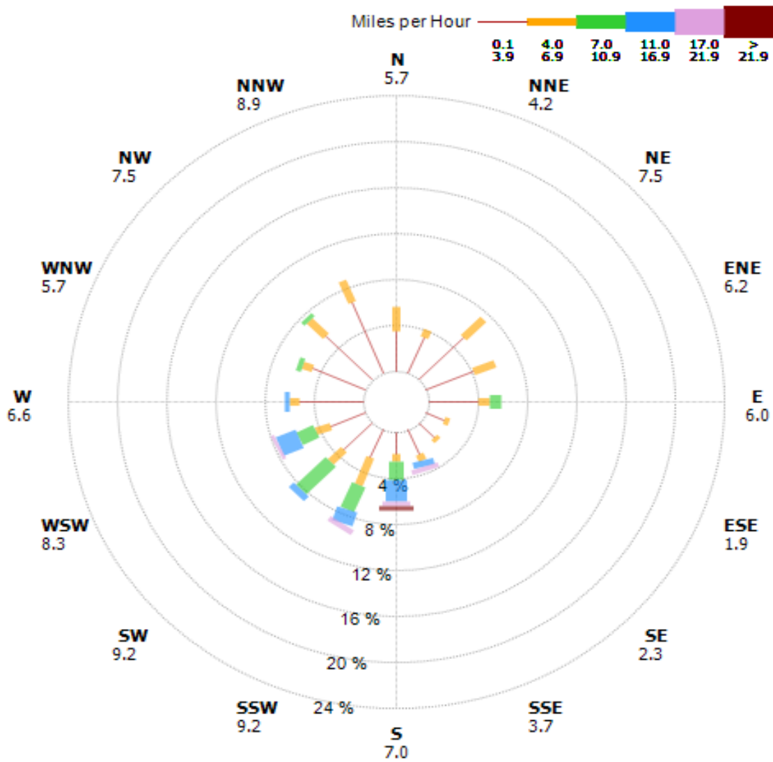
Hour Average Wind Speed Spokane E Ferry ~ 696 Observations 01 Nov 2007 through 30 Nov 2007
