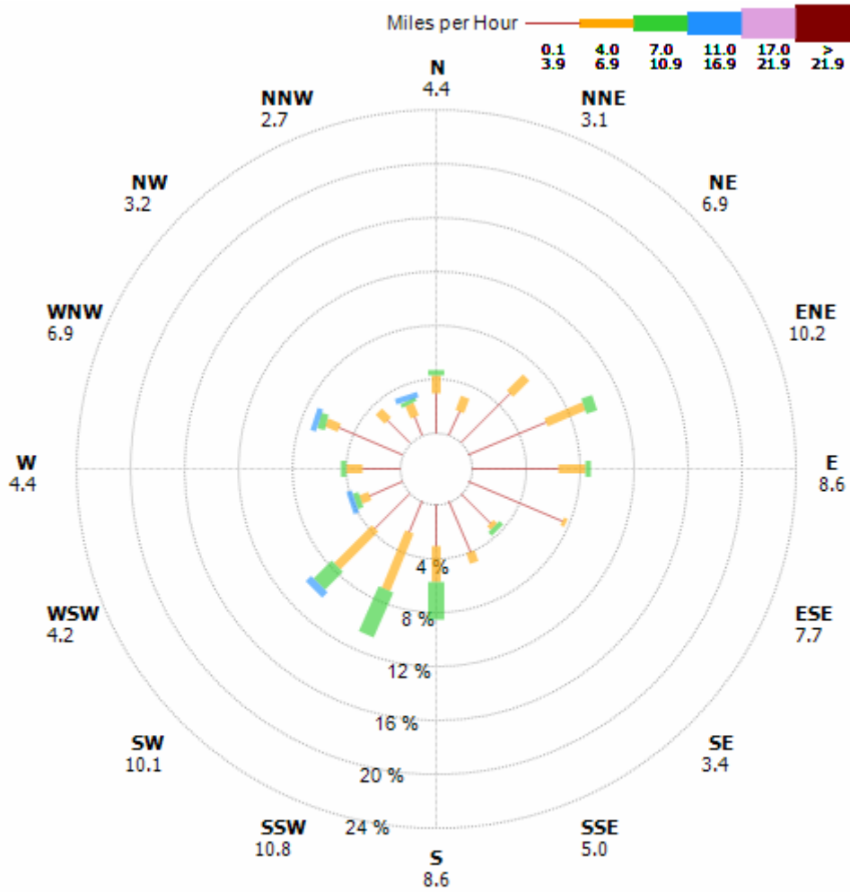
Hour Average Wind Speed Spokane E Ferry ~ 744 Observations 01 Oct 2006 through 31 Oct 2006
