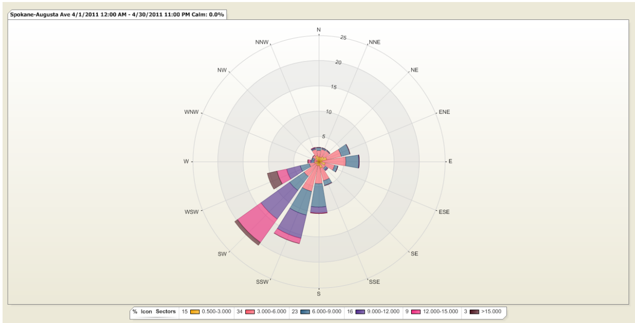
Figure 3: The wind rose depicts the variation of hourly average wind speed (mph) with the direction from which the wind was blowing in April.
