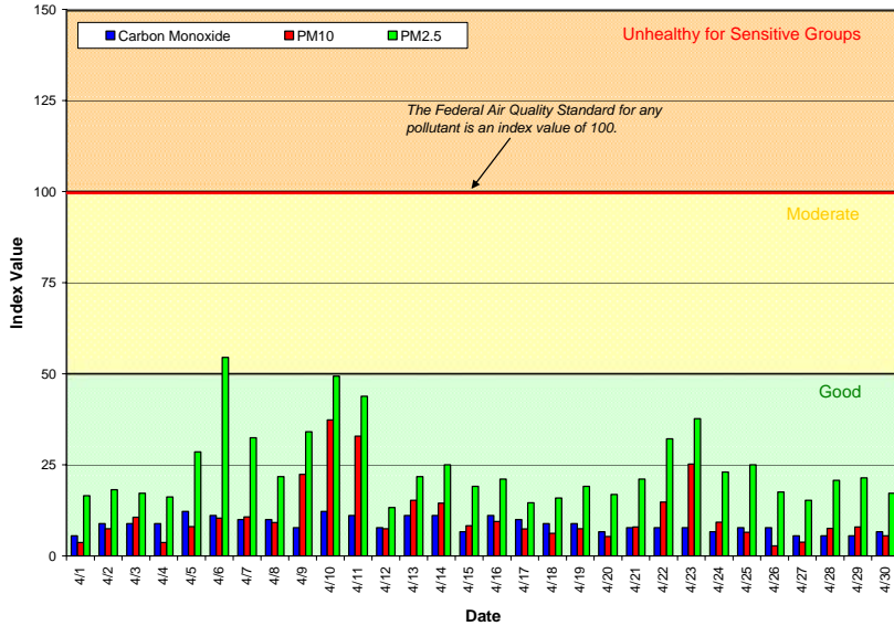
Figure 1: Air Quality Index (AQI) values for April 2012
