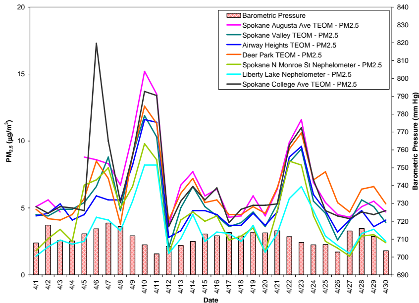
Figure 2: PM 2.5 multi-station time series for April 2012
