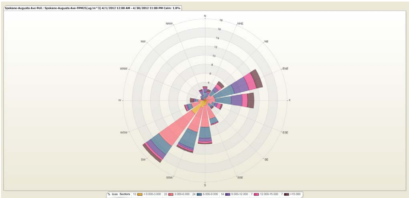
Figure 4: The PM 2.5 pollution rose depicts the variation of hourly average PM 2.5 (µg/m 3 ) with the direction from which the wind was blowing in April.
