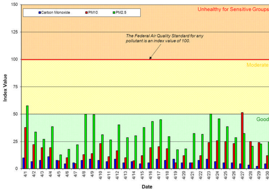
Figure 1: Air Quality Index (AQI) values for April 2013
