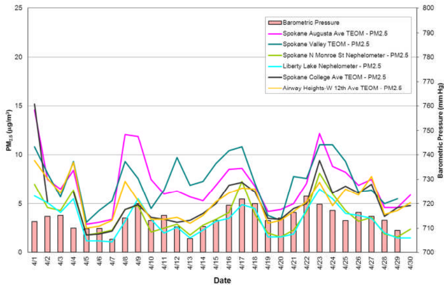
Figure 2: PM 2.5 multi-station time series for April 2013
