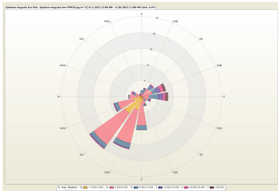
Figure 4: The PM 2.5 pollution rose depicts the variation of hourly average PM 2.5 ( \mu\text{g}/\text{m}^3 ) with the direction from which the wind was blowing in April.
