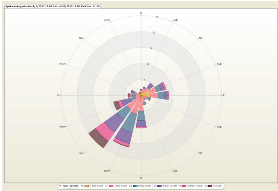
Figure 3: The wind rose depicts the variation of hourly average wind speed (mph) with the direction from which the wind was blowing in April.
