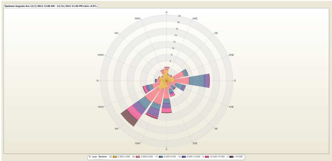
Figure 3: The wind rose depicts the variation of hourly average wind speed (mph) with the direction from which the wind was blowing in December.
