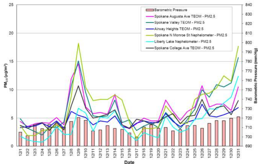
Figure 2: PM 2.5 multi-station time series for December 2012
