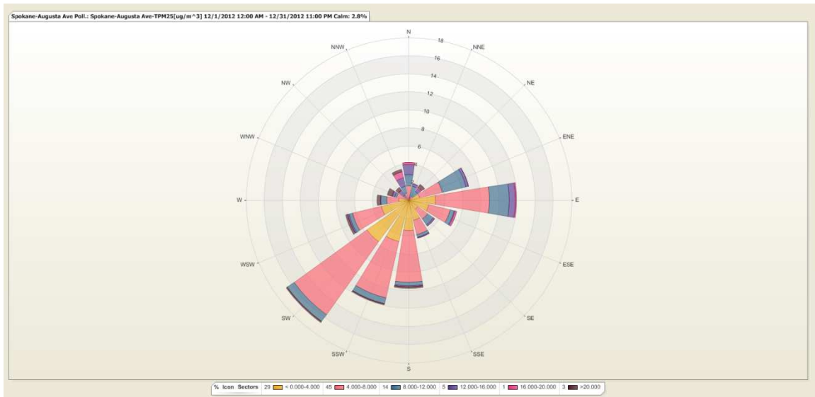
Figure 4: The PM 2.5 pollution rose depicts the variation of hourly average PM 2.5 (µg/m 3 ) with the direction from which the wind was blowing in December.
