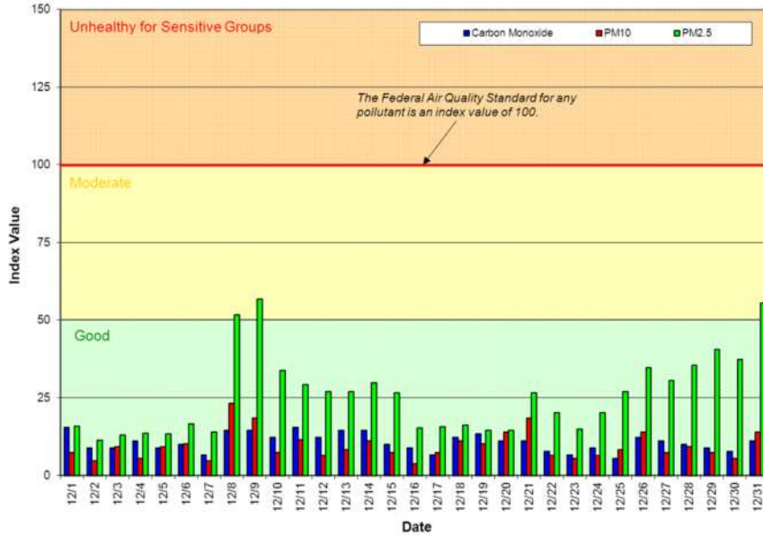
Figure 1: Air Quality Index (AQI) values for December 2012
