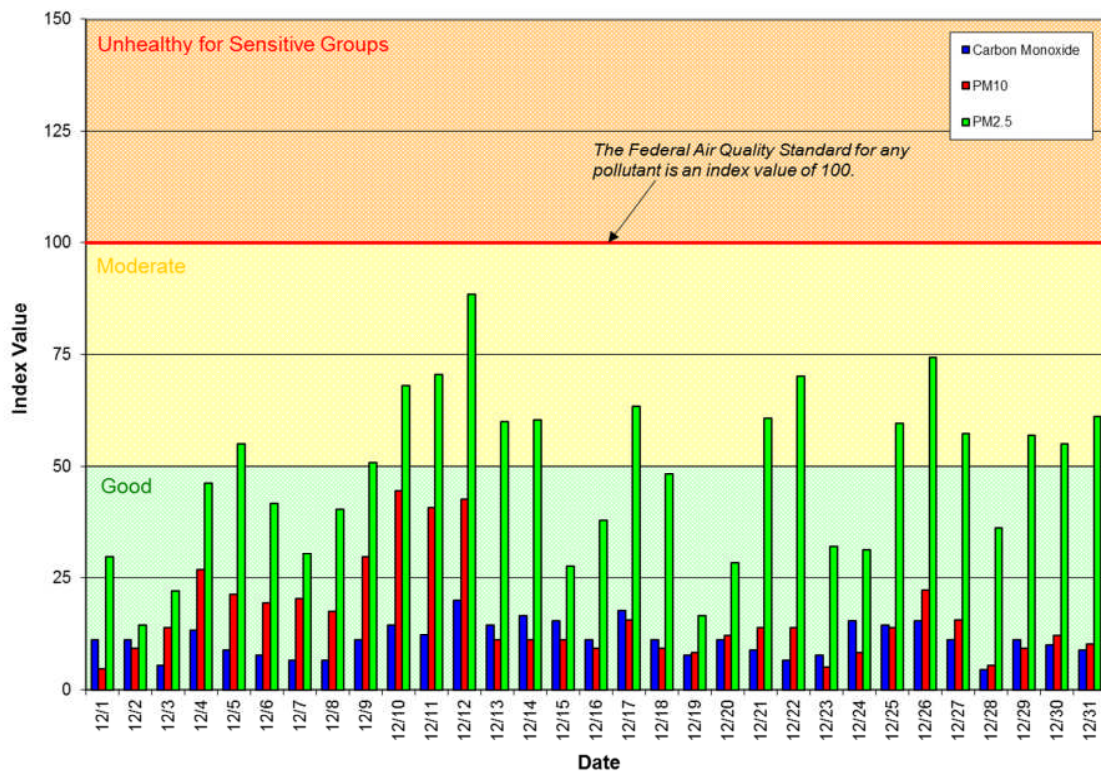
Figure 1: Air Quality Index (AQI) values for December 2013
