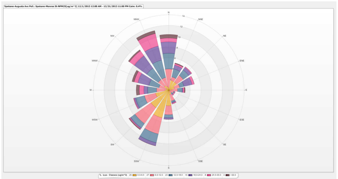
Figure 4: The PM 2.5 pollution rose depicts the variation of hourly average PM 2.5 ( \mu\text{g}/\text{m}^3 ) with the direction from which the wind was blowing in December.
