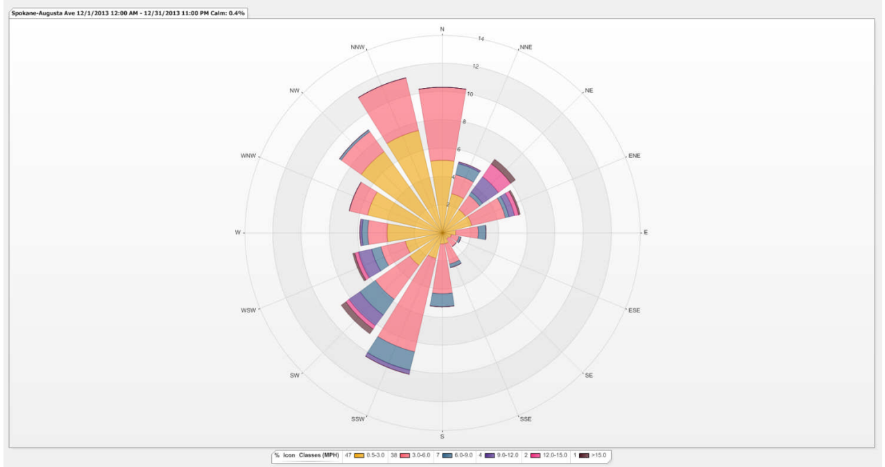
Figure 3: The wind rose depicts the variation of hourly average wind speed (mph) with the direction from which the wind was blowing in December.
