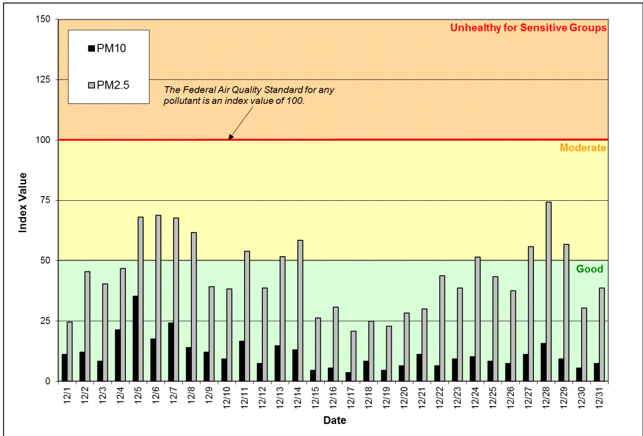
Figure 1: Air Quality Index (AQI) values for December 2017. The data represent the maximum AQI values across all monitoring stations within Spokane County.
