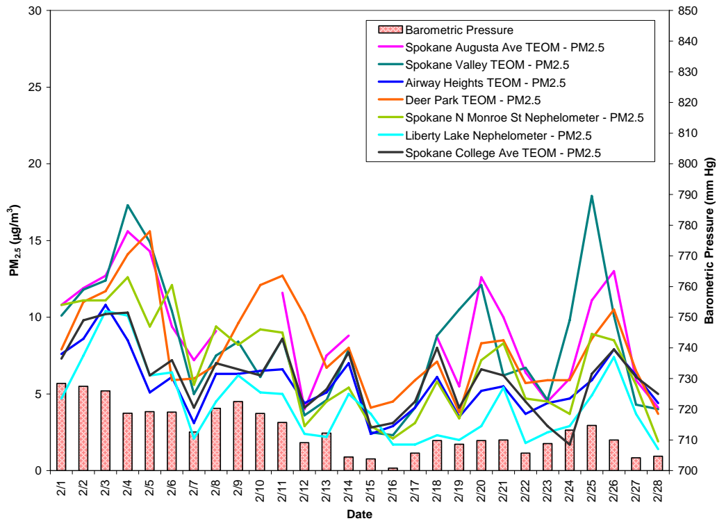
Figure 2: PM 2.5 multi-station time series for February 2011
