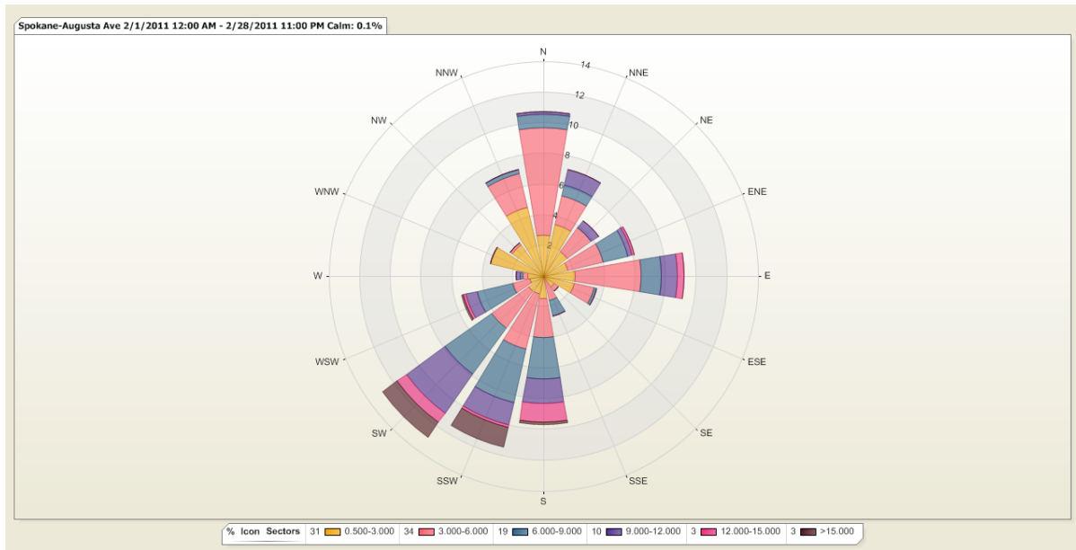
Figure 3: The wind rose depicts the variation of hourly average wind speed (mph) with the direction from which the wind was blowing in February.
