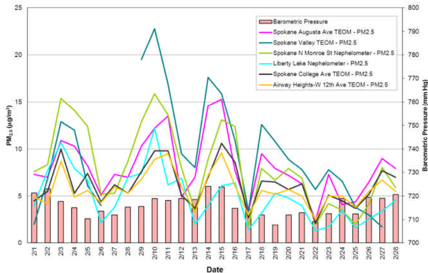
Figure 2: PM 2.5 multi-station time series for February 2013
