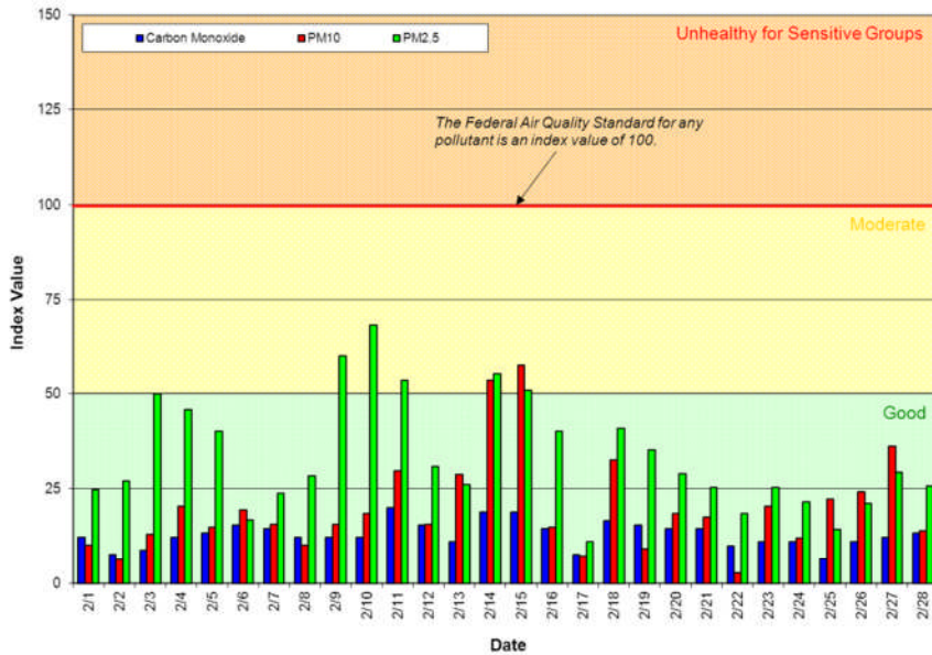
Figure 1: Air Quality Index (AQI) values for February 2013
