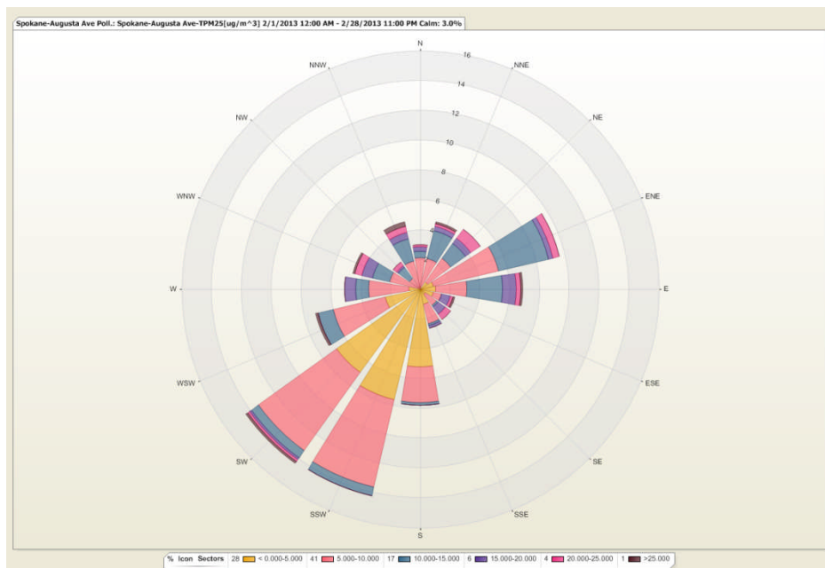
Figure 4: The PM 2.5 pollution rose depicts the variation of hourly average PM 2.5 ( \mu\text{g}/\text{m}^3 ) with the direction from which the wind was blowing in February.
