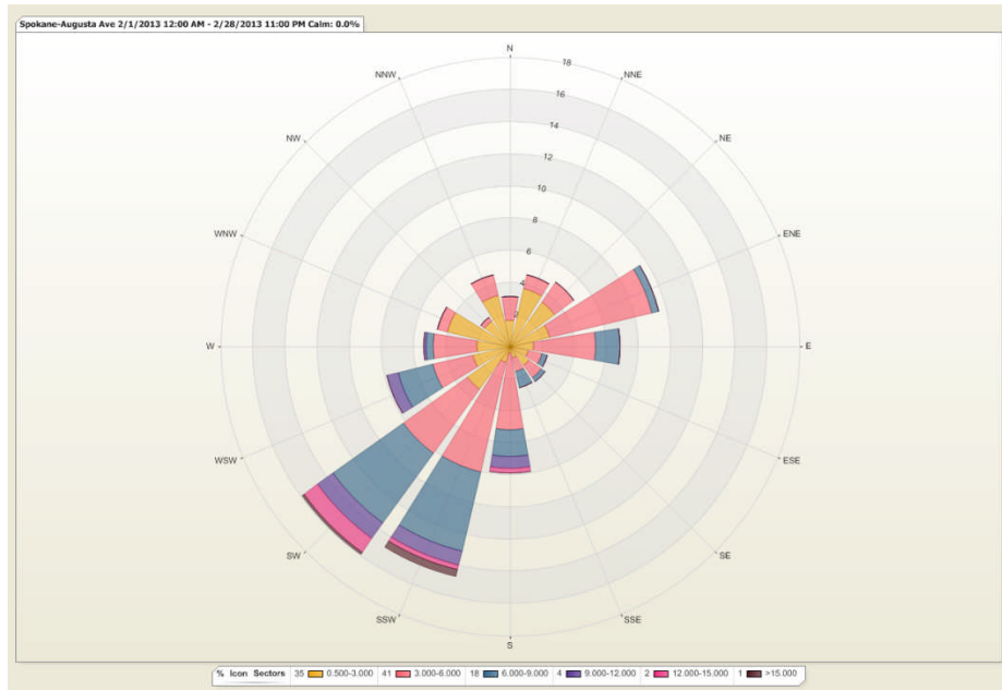
Figure 3: The wind rose depicts the variation of hourly average wind speed (mph) with the direction from which the wind was blowing in February.
