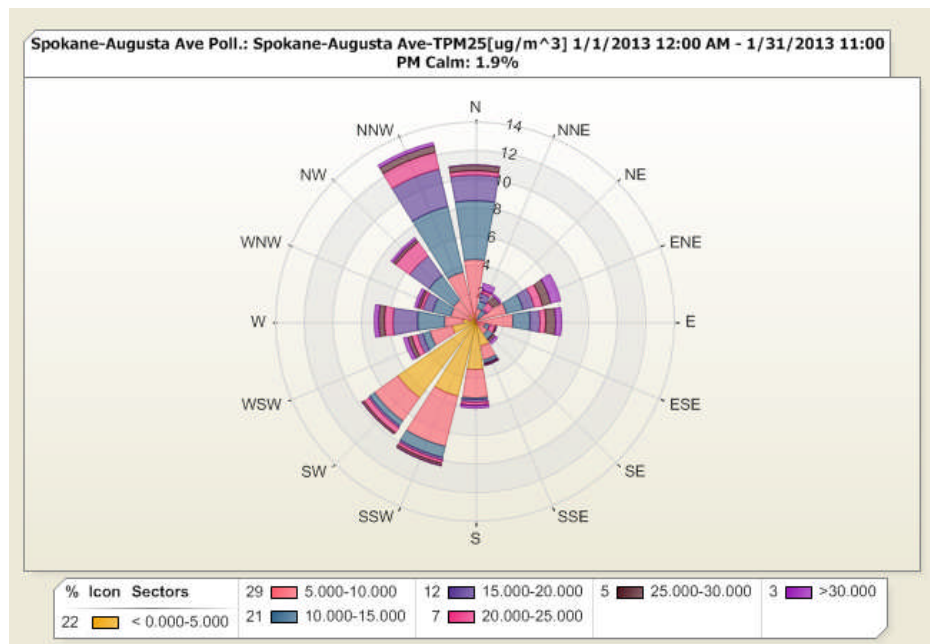
Figure 4: The PM 2.5 pollution rose depicts the variation of hourly average PM 2.5 (µg/m 3 ) with the direction from which the wind was blowing in January.
