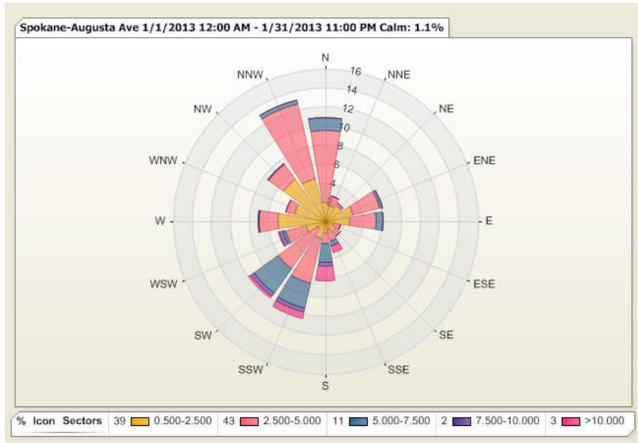
Figure 3: The wind rose depicts the variation of hourly average wind speed (mph) with the direction from which the wind was blowing in January.
