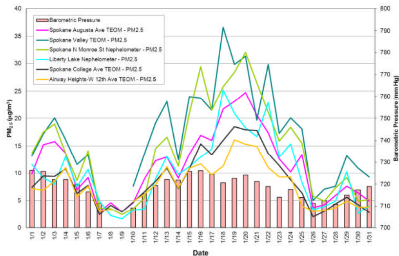
Figure 2: PM 2.5 multi-station time series for January 2013
