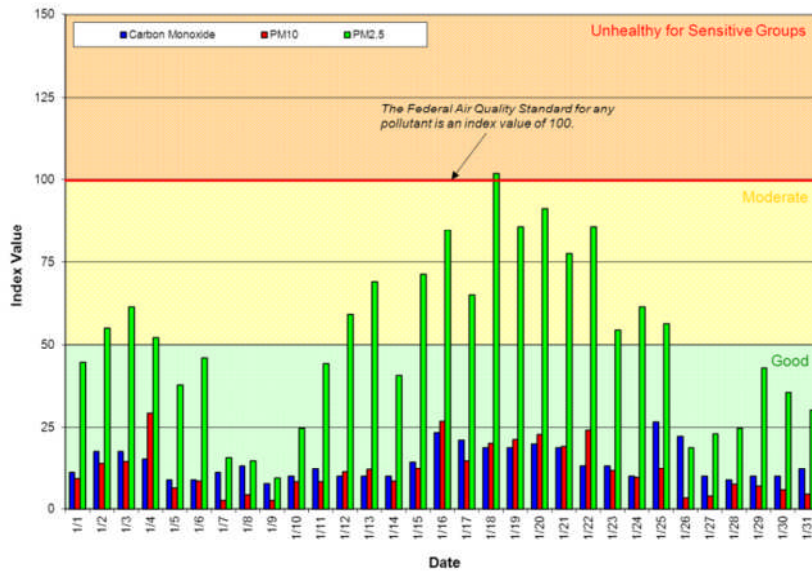
Figure 1: Air Quality Index (AQI) values for January 2013
