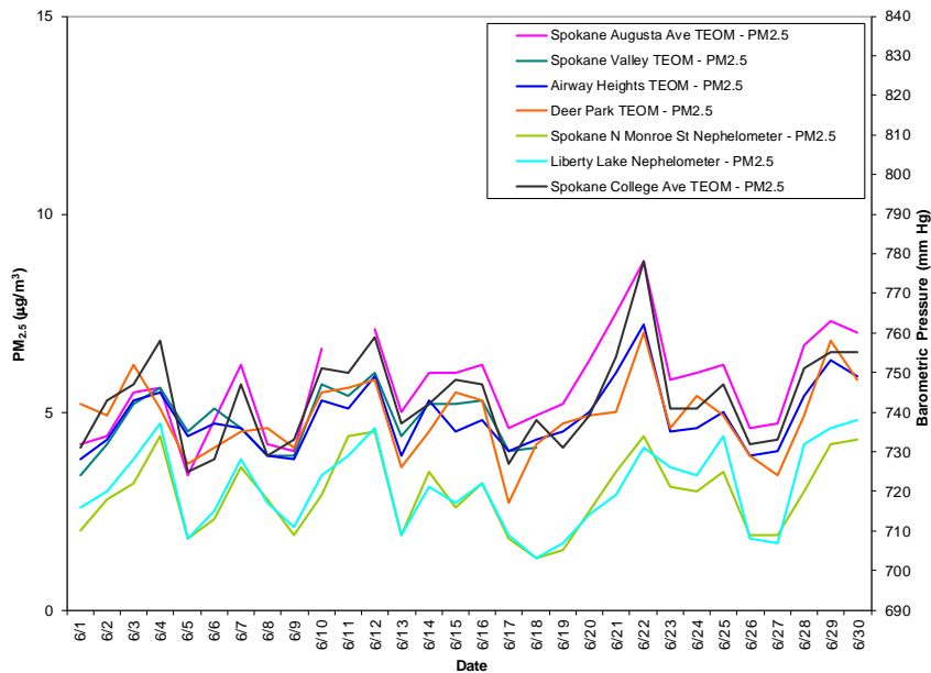
Figure 2: PM 2.5 multi-station time series for June 2012
