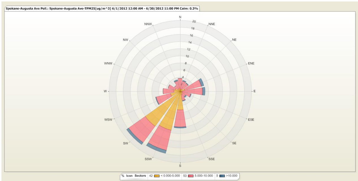
Figure 4: The PM 2.5 pollution rose depicts the variation of hourly average PM 2.5 ( \mu\text{g}/\text{m}^3 ) with the direction from which the wind was blowing in June.
