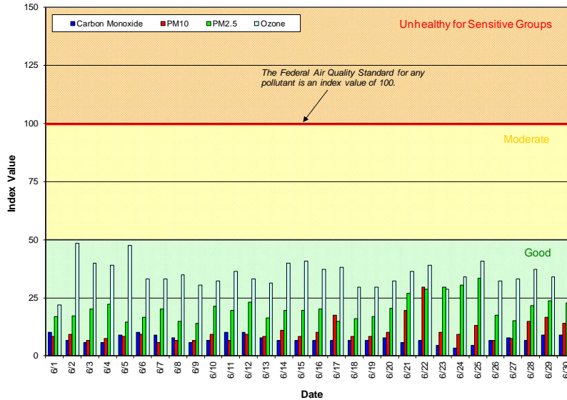
Figure 1: Air Quality Index (AQI) values for June 2012
