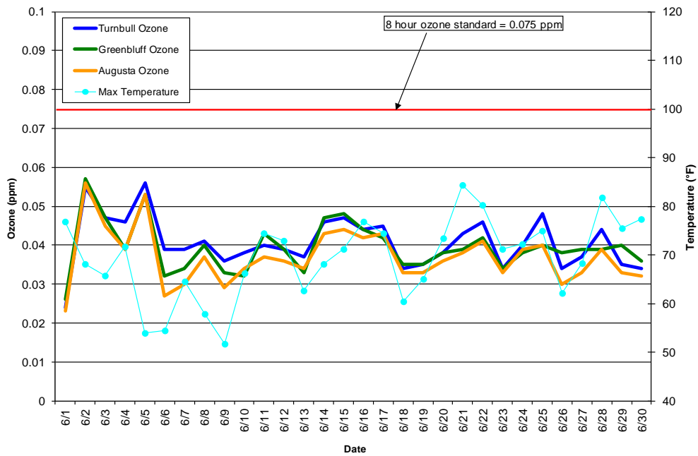
Figure 5: Eight hour maximum ozone concentrations for the Spokane region in June. Daily maximum temperatures are also shown. Daily maximum temperature can be used as a surrogate for solar radiation (ozone is formed through a photochemical reaction) for determining potential ozone maximum concentrations. The threshold for the moderate category for the AQI for ozone is 0.06 ppm averaged over eight hours. An ozone measurement above 0.075 ppm, averaged over eight hours, is the threshold value for the federal ozone standard. It is not a violation of the standard to exceed this level on a given day because determination of attainment status is based on averaging data over a period of years. See Appendix 1 for more detailed information about attainment of federal air quality standards.
