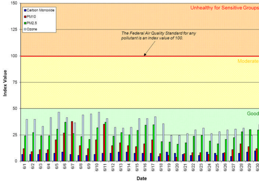
Figure 1: Air Quality Index (AQI) values for June 2013
