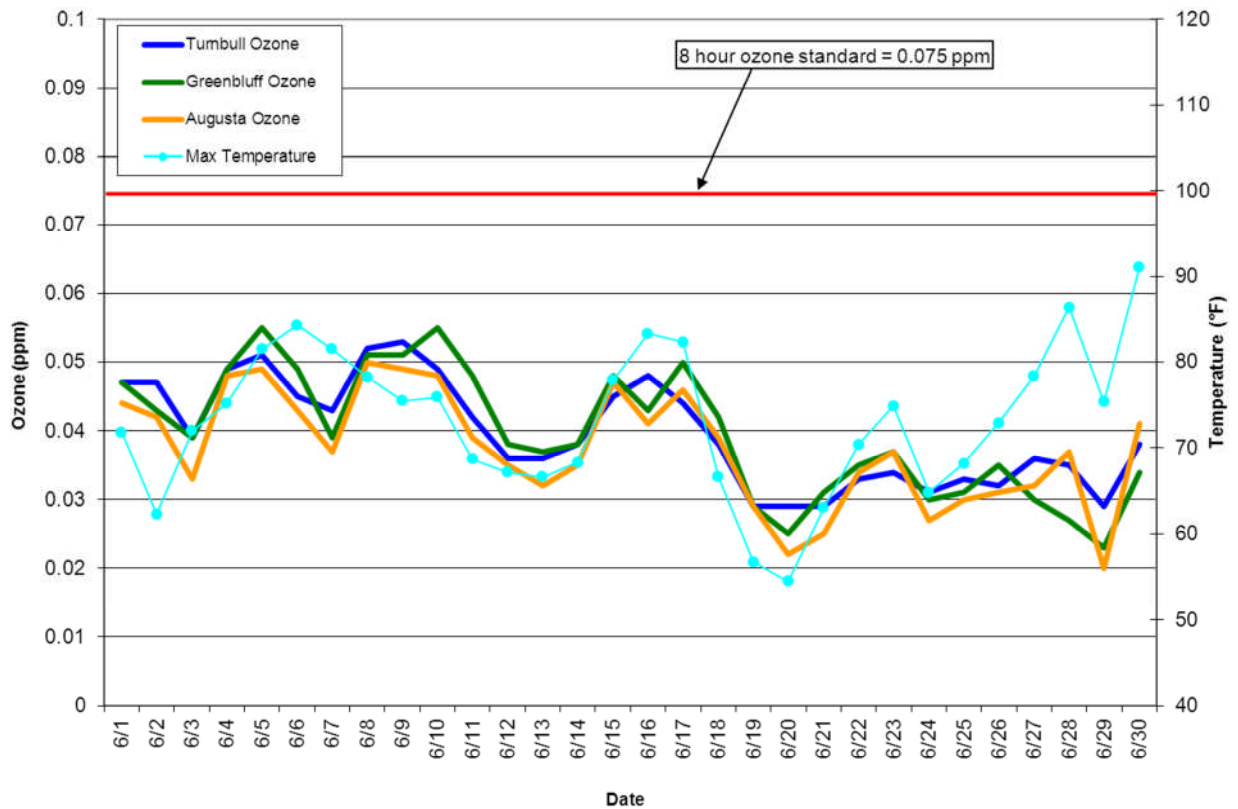
Figure 5: Eight hour maximum ozone concentrations for the Spokane region in June. Daily maximum temperatures are also shown. Daily maximum temperature can be used as a surrogate for solar radiation (ozone is formed through a photochemical reaction) for determining potential ozone maximum concentrations. The threshold for the moderate category for the AQI for ozone is 0.06 ppm averaged over eight hours. An ozone measurement above 0.075 ppm, averaged over eight hours, is the threshold value for the federal ozone standard. It is not a violation of the standard to exceed this level on a given day because determination of attainment status is based on averaging data over a period of years. See Appendix 1 for more detailed information about attainment of federal air quality standards.
