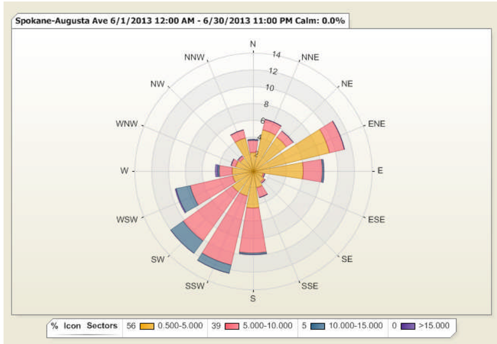
Figure 3: The wind rose depicts the variation of hourly average wind speed (mph) with the direction from which the wind was blowing in June.
