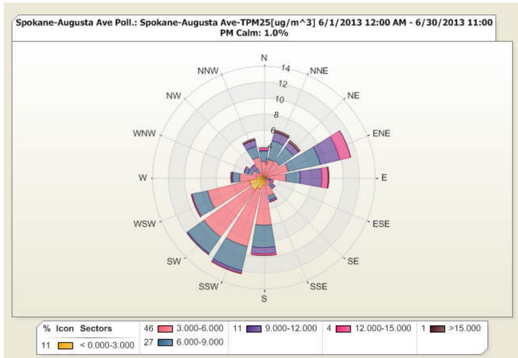
Figure 4: The PM 2.5 pollution rose depicts the variation of hourly average PM 2.5 (µg/m 3 ) with the direction from which the wind was blowing in June.
