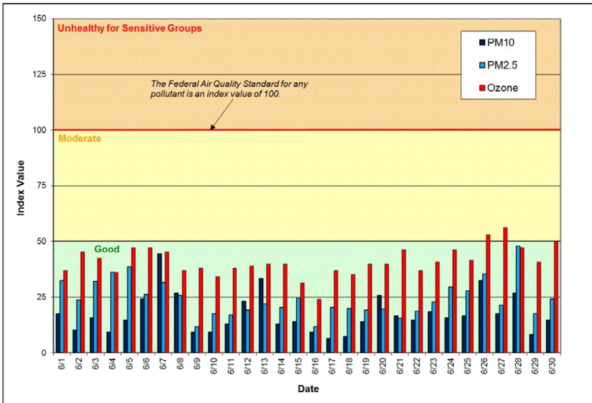
Figure 1: Air Quality Index (AQI) values for June 2017. The data represent the maximum AQI values across all monitoring stations within Spokane County.
