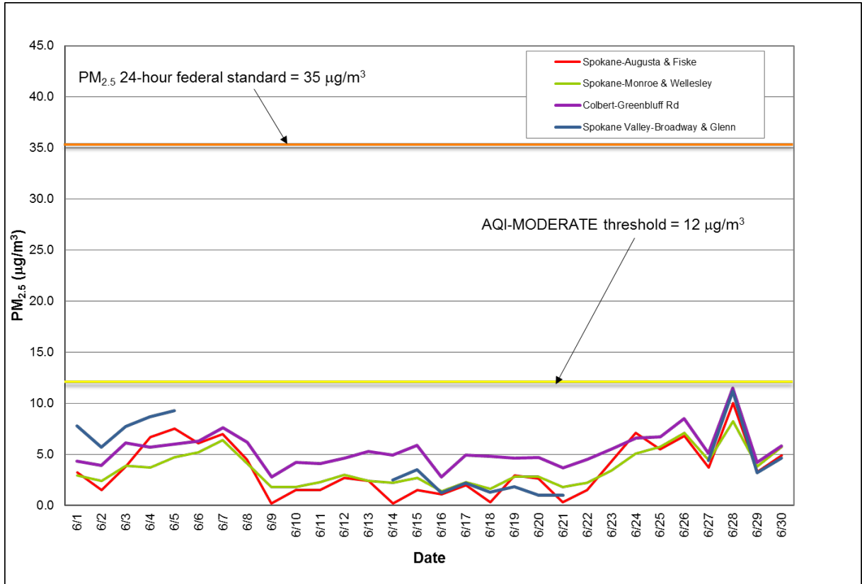
Figure 2: Multi-station 24-hour average PM 2.5 for June 2017; Spokane County.
