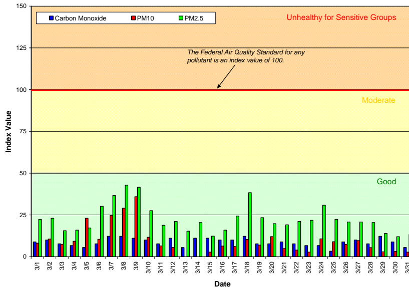
Figure 1: Air Quality Index (AQI) values for March 2012
