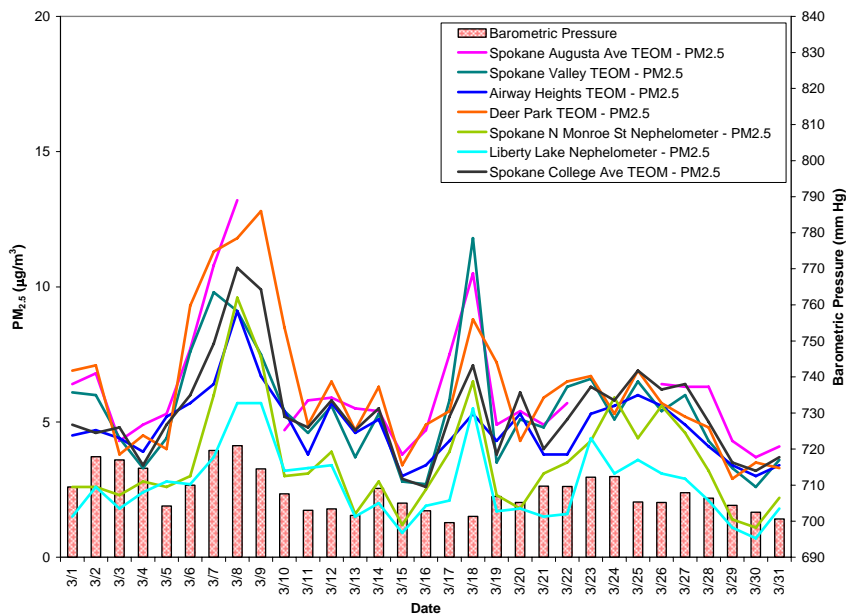
Figure 2: PM 2.5 multi-station time series for March 2012
