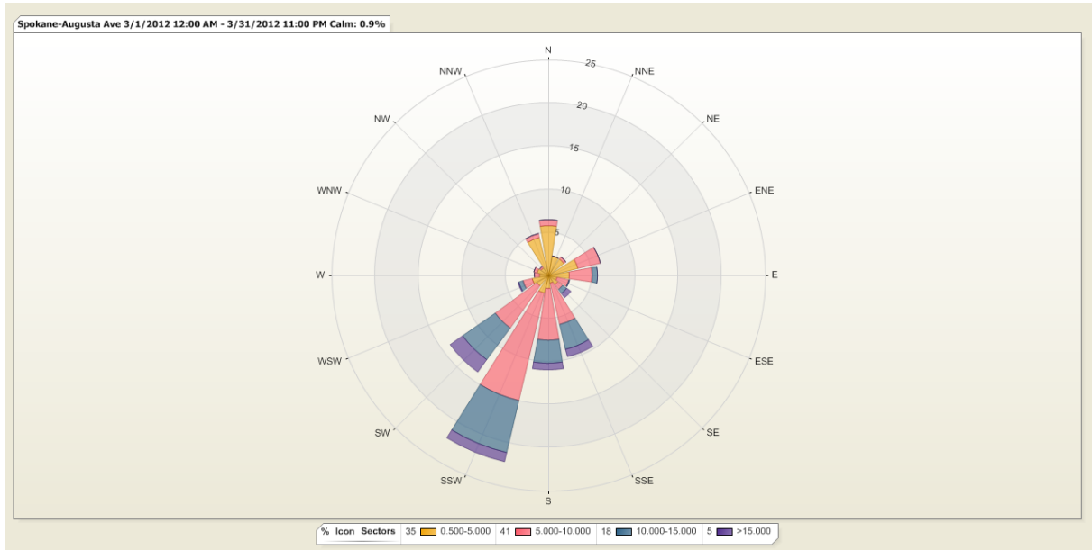
Figure 3: The wind rose depicts the variation of hourly average wind speed (mph) with the direction from which the wind was blowing in March.
