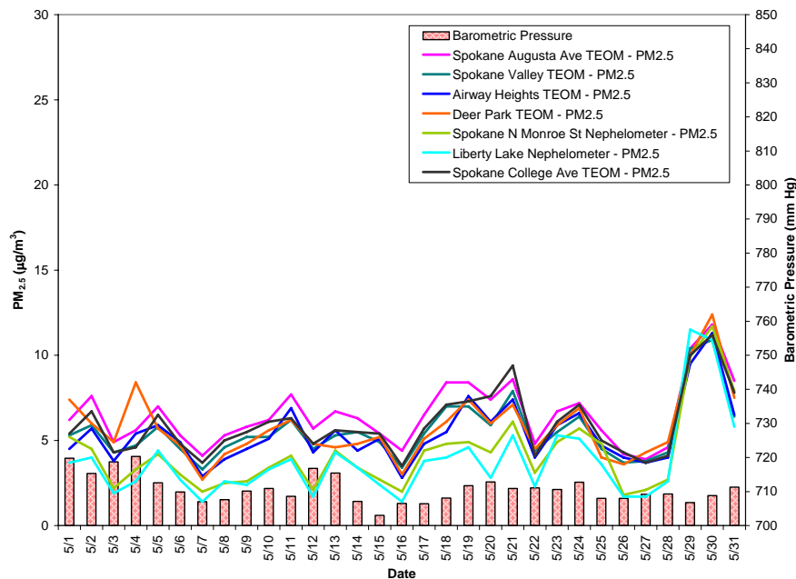
Figure 2: PM 2.5 multi-station time series for May 2011
