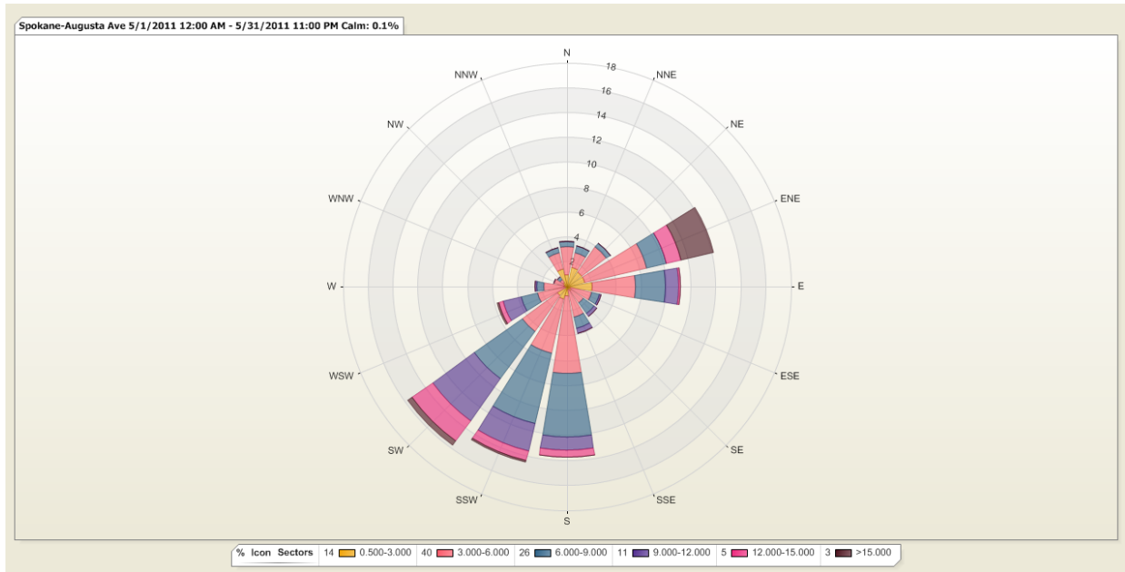
Figure 3: The wind rose depicts the variation of hourly average wind speed (mph) with the direction from which the wind was blowing in May.
