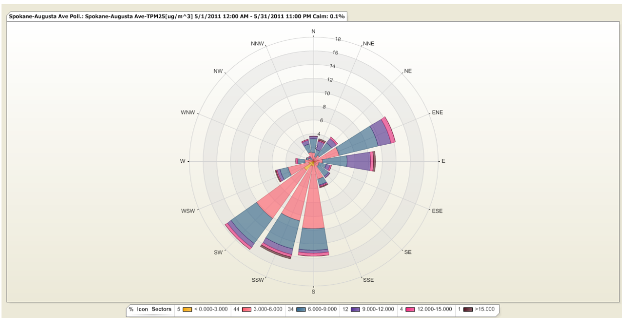
Figure 4: The PM 2.5 pollution rose depicts the variation of hourly average PM 2.5 ( \mu\text{g}/\text{m}^3 ) with the direction from which the wind was blowing in May.
