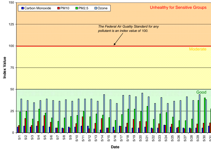
Figure 1: Air Quality Index (AQI) values for May 2011
