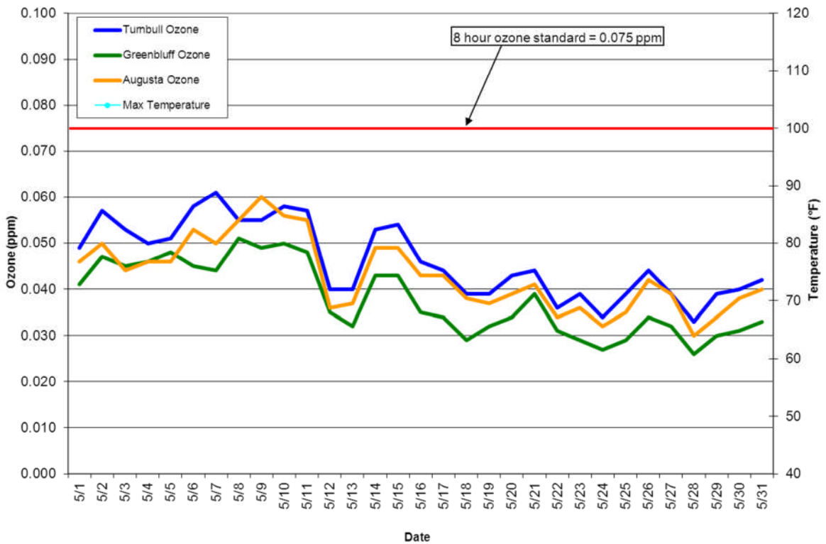
Figure 5: Eight hour maximum ozone concentrations for the Spokane region in May. Daily maximum temperatures are also shown. Daily maximum temperature can be used as a surrogate for solar radiation (ozone is formed through a photochemical reaction) for determining potential ozone maximum concentrations. The threshold for the moderate category for the AQI for ozone is 0.06 ppm averaged over eight hours. An ozone measurement above 0.075 ppm, averaged over eight hours, is the threshold value for the federal ozone standard. It is not a violation of the standard to exceed this level on a given day because determination of attainment status is based on averaging data over a period of years. See Appendix 1 for more detailed information about attainment of federal air quality standards. There are gaps in the ozone data represented on this chart when analyzers were out of calibration.
