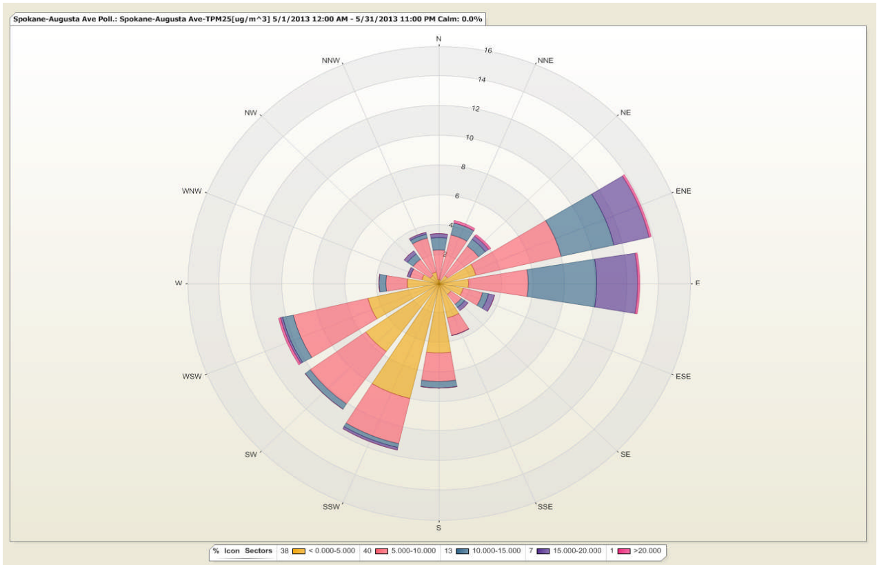
Figure 4: The PM 2.5 pollution rose depicts the variation of hourly average PM 2.5 ( \mu\text{g}/\text{m}^3 ) with the direction from which the wind was blowing in May.
