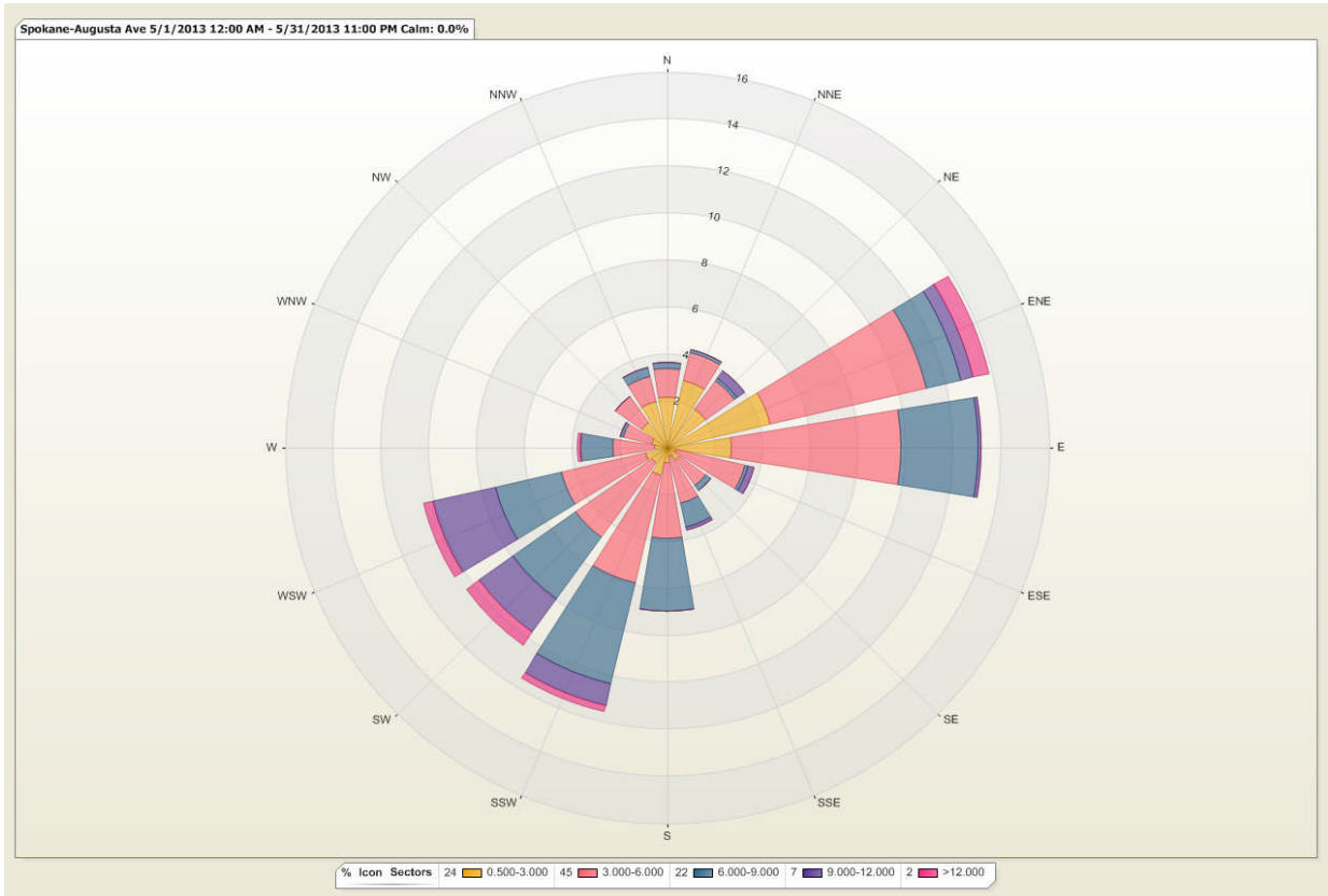
Figure 3: The wind rose depicts the variation of hourly average wind speed (mph) with the direction from which the wind was blowing in May.
