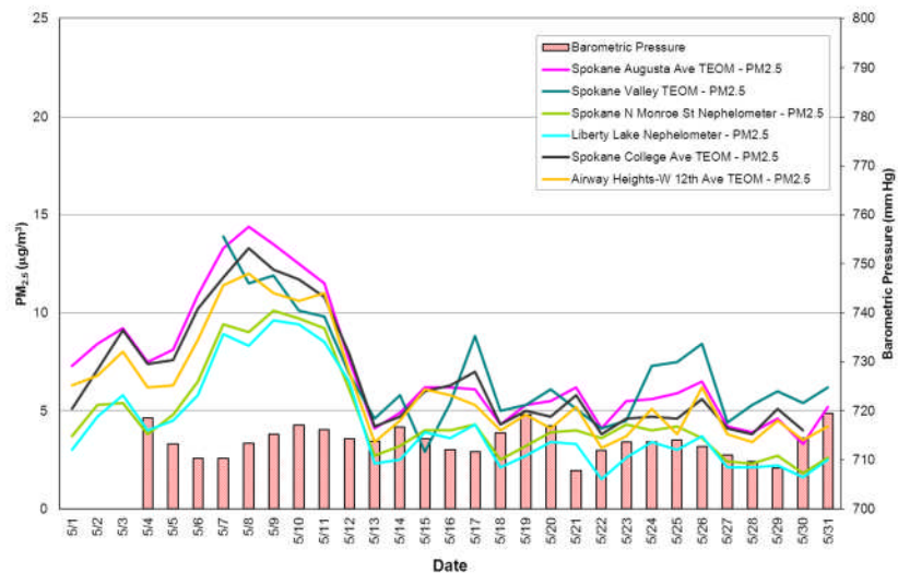
Figure 2: PM 2.5 multi-station time series for May 2013
