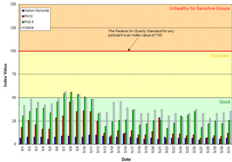
Figure 1: Air Quality Index (AQI) values for May 2013
