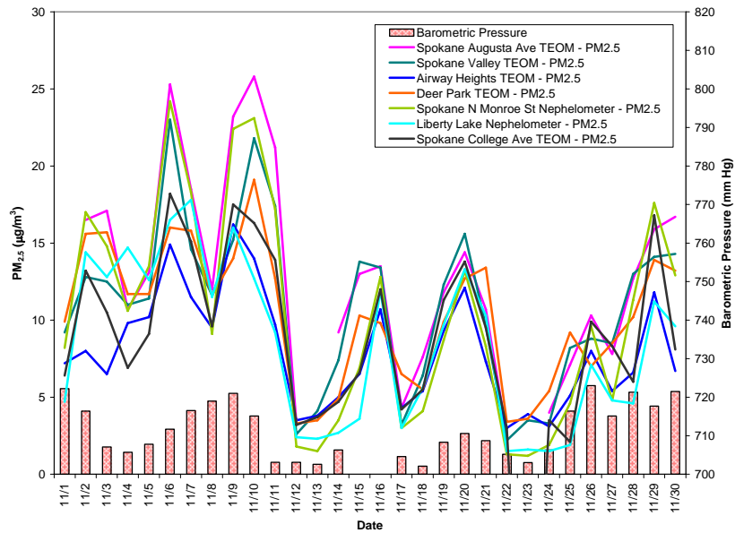
Figure 2: PM 2.5 multi-station time series for November 2011
