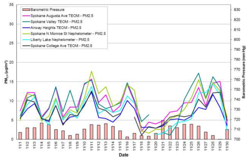
Figure 2: PM 2.5 multi-station time series for November 2012
