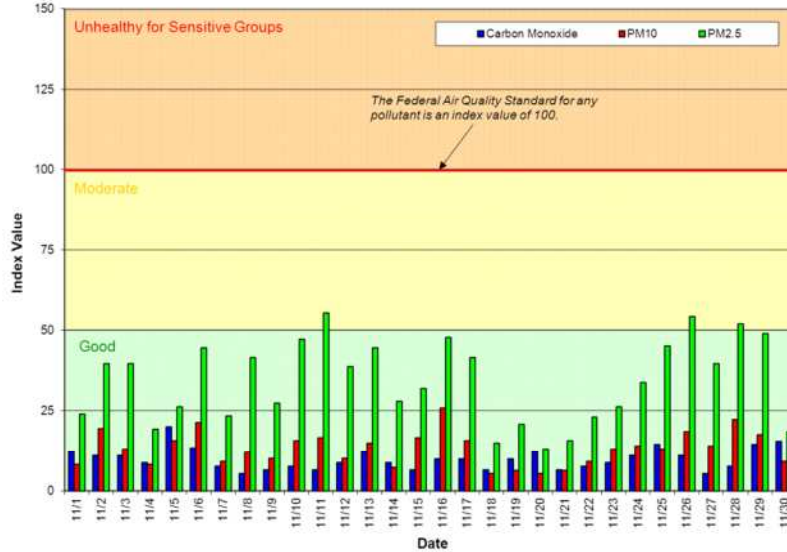
Figure 1: Air Quality Index (AQI) values for November 2012
