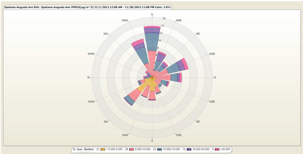
Figure 4: The PM 2.5 pollution rose depicts the variation of hourly average PM 2.5 ( \mu\text{g}/\text{m}^3 ) with the direction from which the wind was blowing in November.
