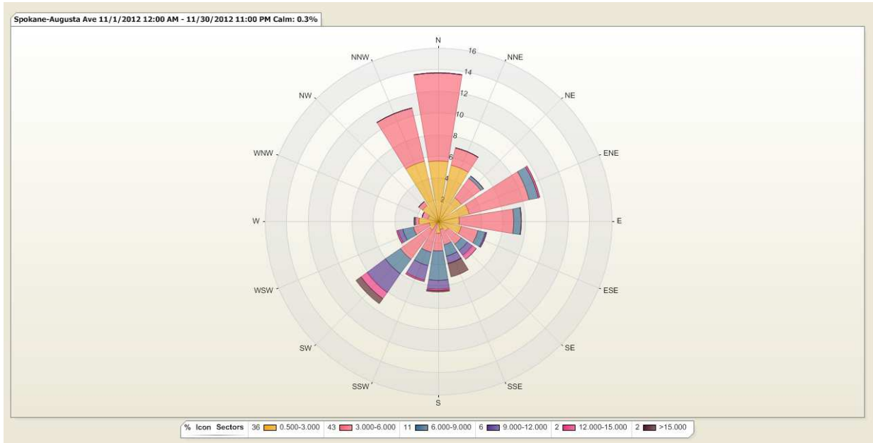
Figure 3: The wind rose depicts the variation of hourly average wind speed (mph) with the direction from which the wind was blowing in November.
