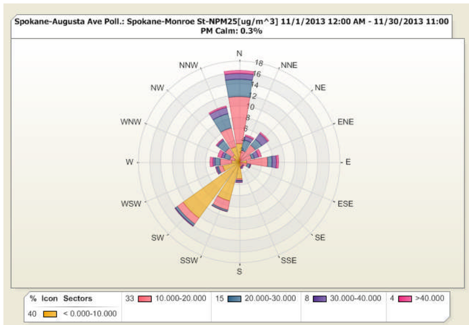
Figure 4: The PM 2.5 pollution rose depicts the variation of hourly average PM 2.5 ( \mu\text{g}/\text{m}^3 ) with the direction from which the wind was blowing in November.
