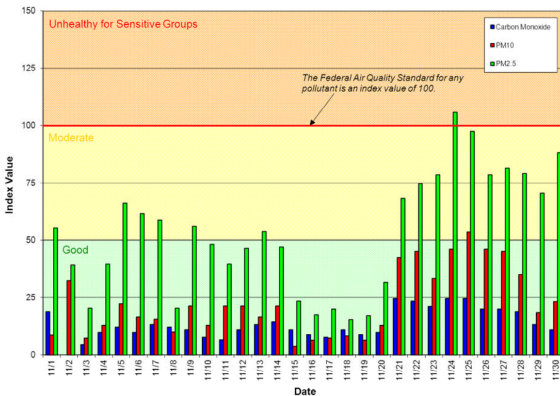
Figure 1: Air Quality Index (AQI) values for November 2013
