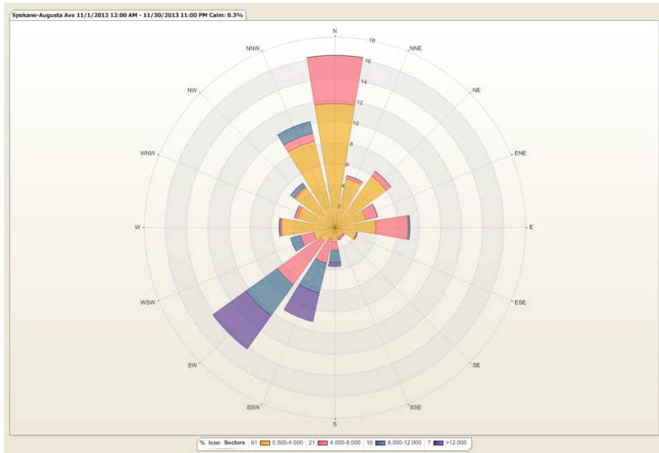
Figure 3: The wind rose depicts the variation of hourly average wind speed (mph) with the direction from which the wind was blowing in November.
