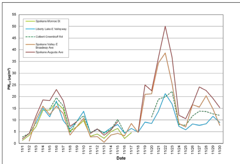
Figure 2: Multi-station 24-hour average PM 2.5 for November 2015; Spokane County.
