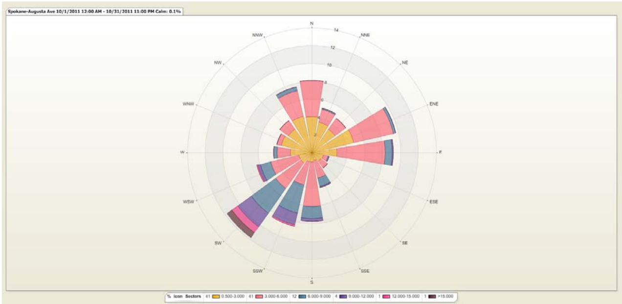
Figure 3: The wind rose depicts the variation of hourly average wind speed (mph) with the direction from which the wind was blowing in October.
