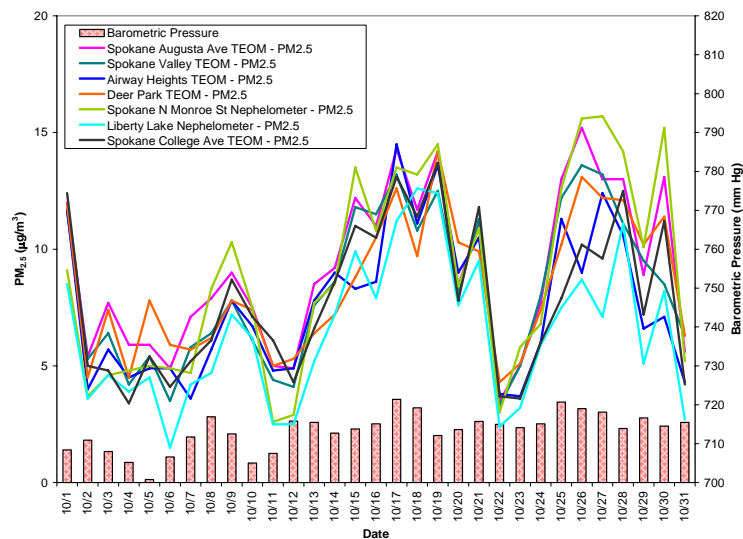
Figure 2: PM 2.5 multi-station time series for October 2011
