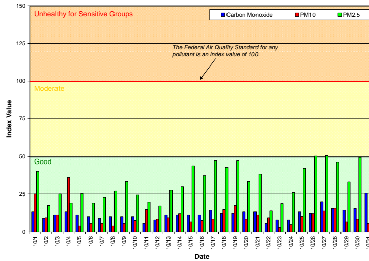
Figure 1: Air Quality Index (AQI) values for October 2011
