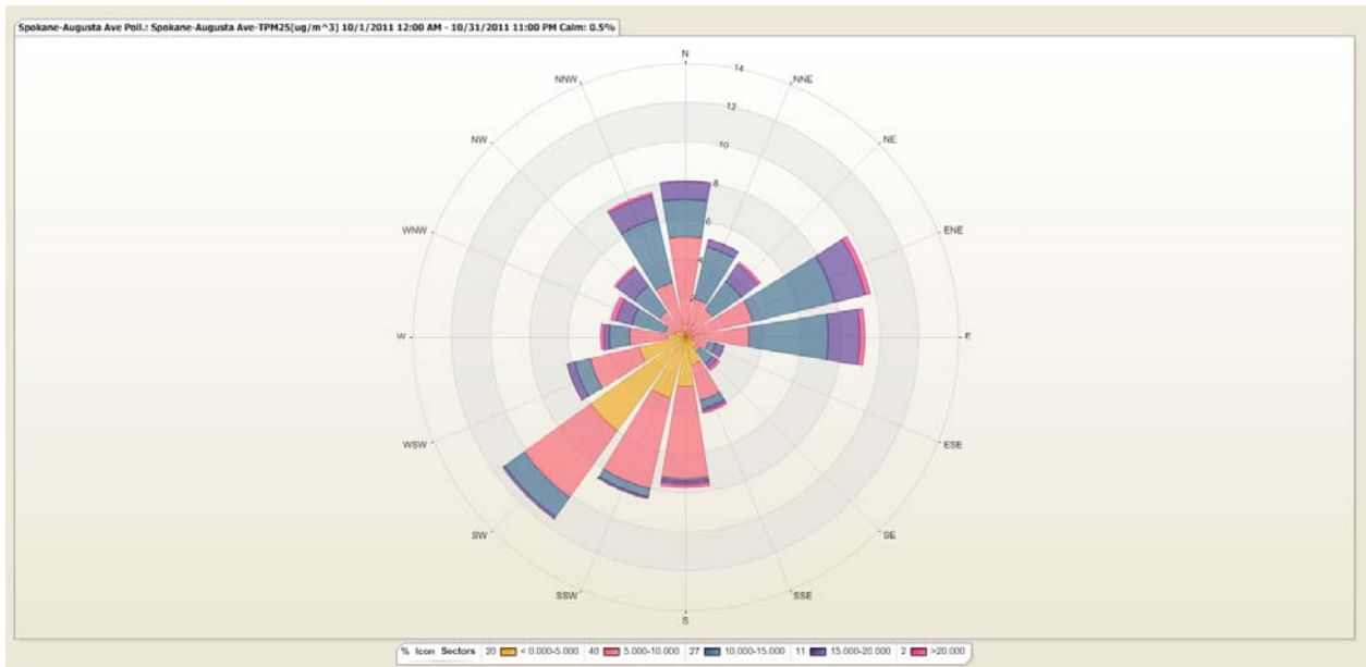
Figure 4: The PM 2.5 pollution rose depicts the variation of hourly average PM 2.5 (µg/m 3 ) with the direction from which the wind was blowing in October.
