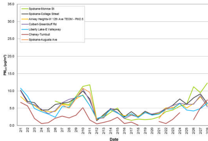
Figure 2: PM 2.5 multi-station time series for February 2014
