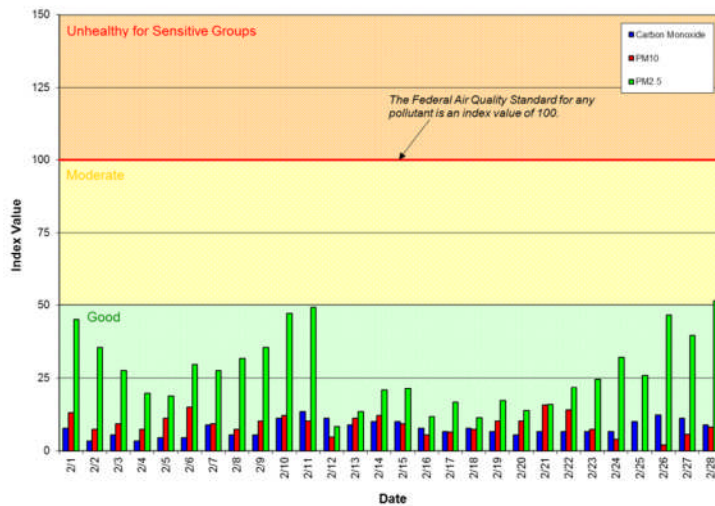
Figure 1: Air Quality Index (AQI) values for February 2014
