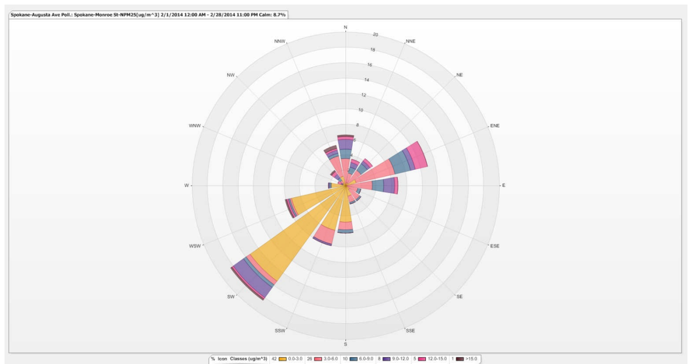
Figure 4: The PM 2.5 pollution rose depicts the variation of hourly average PM 2.5 (µg/m 3 ) with the direction from which the wind was blowing in February.
