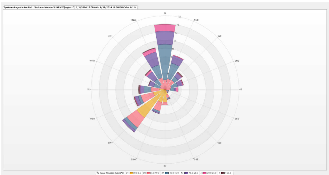
Figure 4: The PM_{2.5} pollution rose depicts the variation of hourly average PM_{2.5} ( \mu g/m^3 ) with the direction from which the wind was blowing in January.
