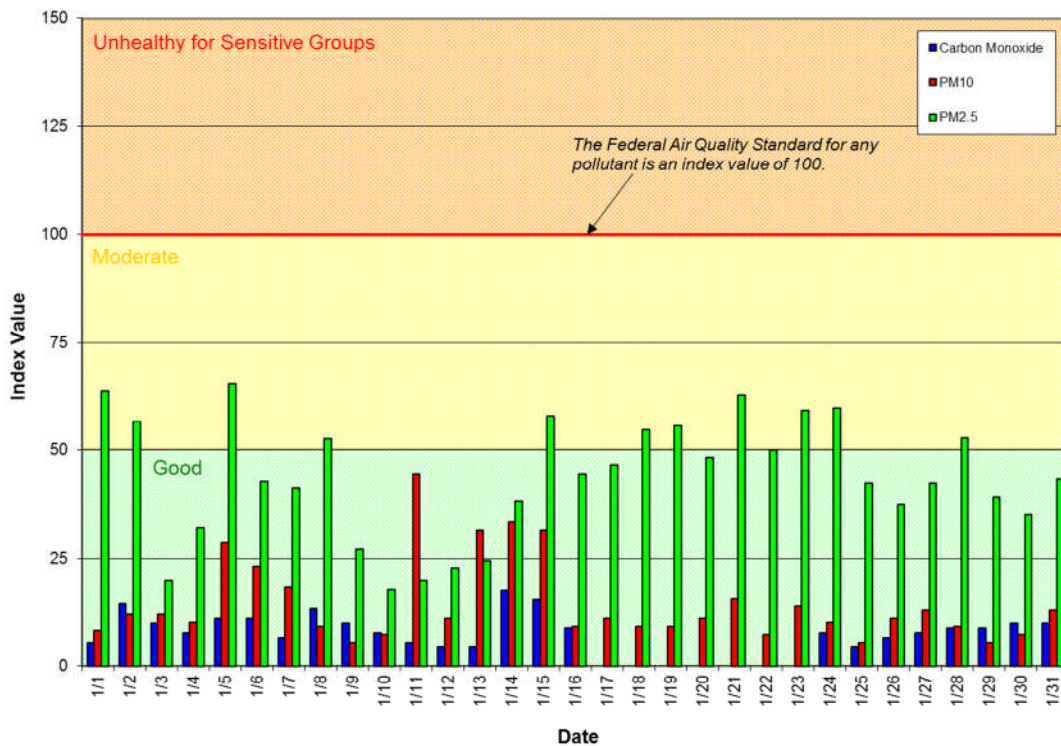
Figure 1: Air Quality Index (AQI) values for January 2014
