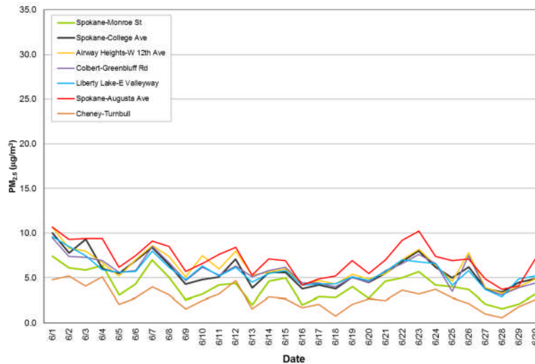
Figure 2: PM 2.5 multi-station time series for June 2014.
