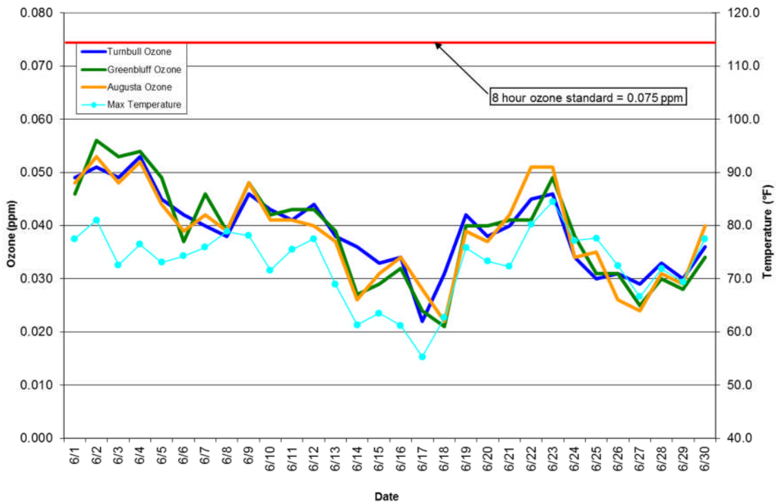
Figure 5: Eight hour maximum ozone concentrations for the Spokane region in June. Daily 1-hour maximum temperatures are also shown. Daily maximum temperature can be used as a surrogate for solar radiation (ozone is formed through a photochemical reaction) for determining potential ozone maximum concentrations. The threshold for the moderate category of the AQI for ozone is 0.06 ppm averaged over eight hours. An ozone measurement above 0.075 ppm, averaged over eight hours, is the threshold value for the federal ozone standard. It is not a violation of the standard to exceed this level on a given day because determination of attainment status is based on averaging data over a period of years. See Appendix 1 for more detailed information about attainment of federal air quality standards.
