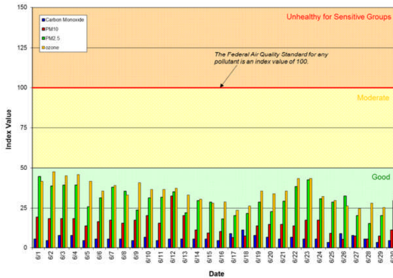
Figure 1: Air Quality Index (AQI) values for June 2014
