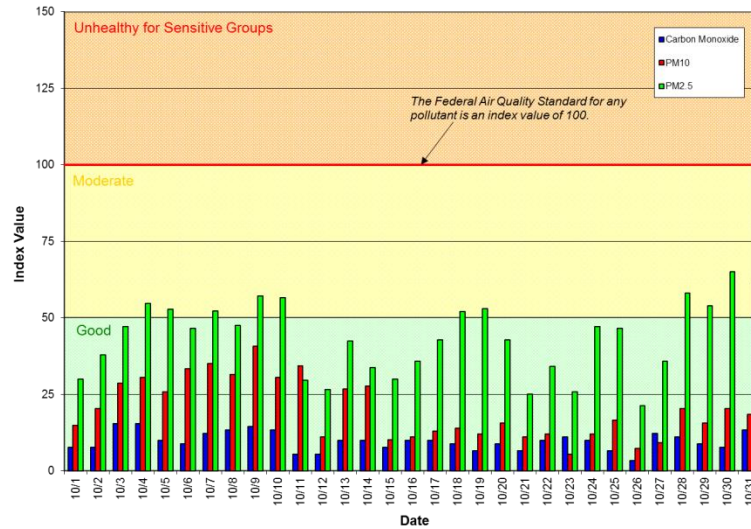
Figure 1: Air Quality Index (AQI) values for October 2014. The data represent the maximum AQI values across all monitoring stations within Spokane County.
