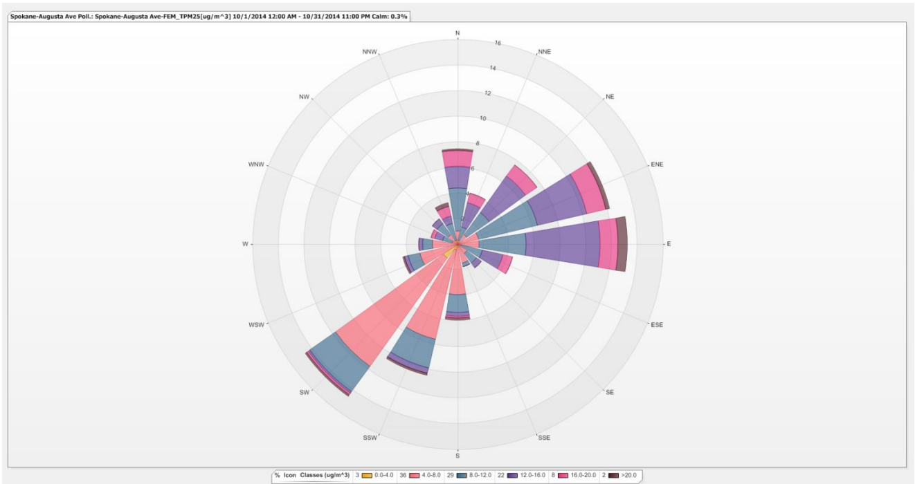
Figure 4: The PM 2.5 pollution rose depicts the variation of hourly average PM 2.5 (µg/m 3 ) with the direction from which the wind was blowing in October.
