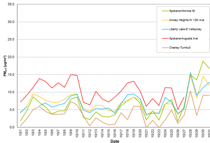
Figure 2: Multi-station 24-hour average PM 2.5 for October 2014; Spokane County.
