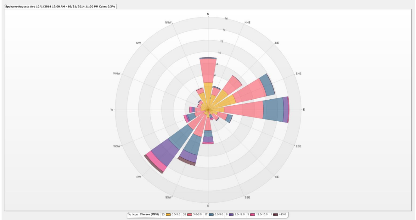
Figure 3: The wind rose depicts the variation of hourly average wind speed (mph) with the direction from which the wind was blowing in October.
